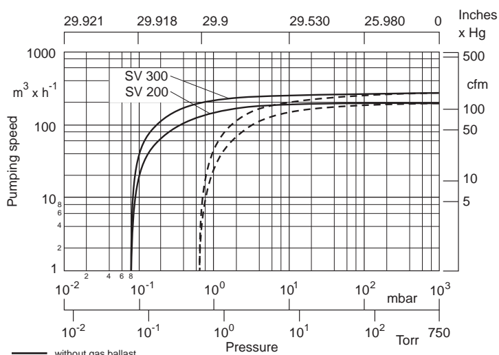
Pumping speed characteristics for the SOGEVAC SV 200 and SV 300 at 60 Hz
