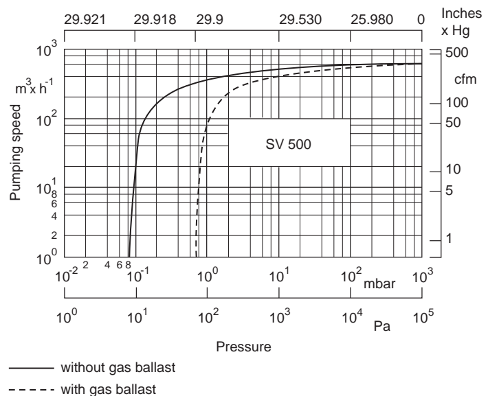
Pumping speed characteristics of the SOGEVAC SV 500 at 50 Hz (60 Hz curves at the end of the section)
